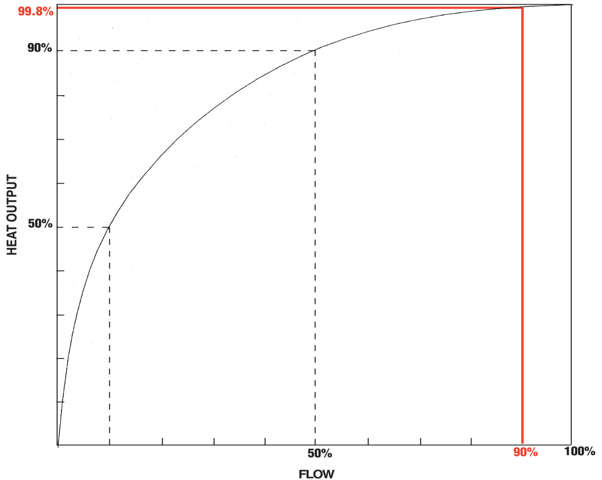
FIG. 17 1996 ASHRAE HANDBOOK; HVAC SYSTEMS AND EQUIPMENT
