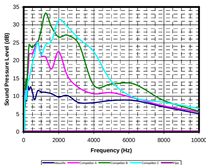
Noise Produced at 4 psi Differential Pressure
