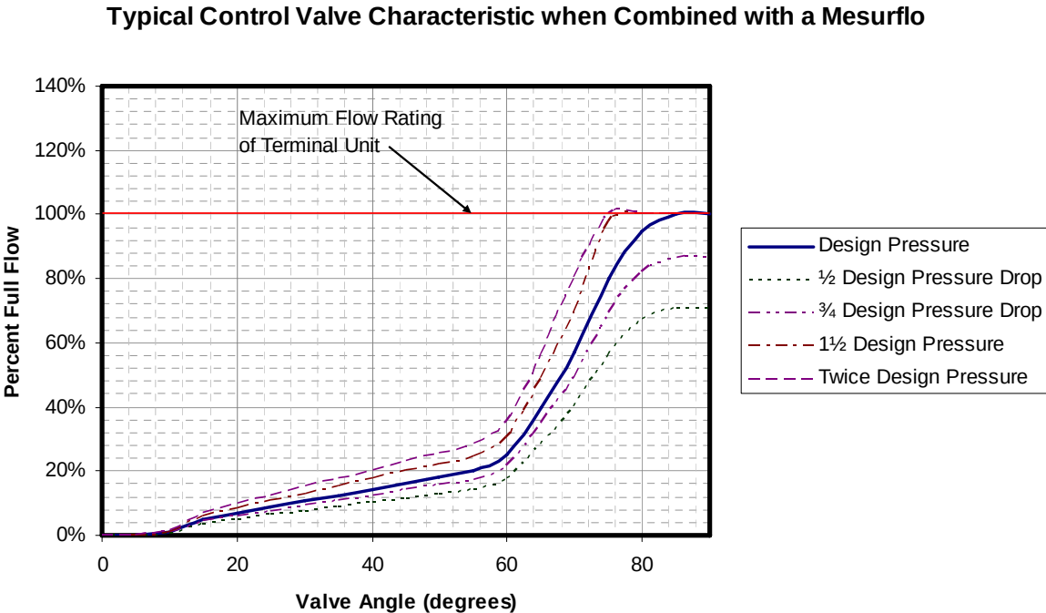
Figure E: Performance of a Modulating Control valve with Mesurflo
