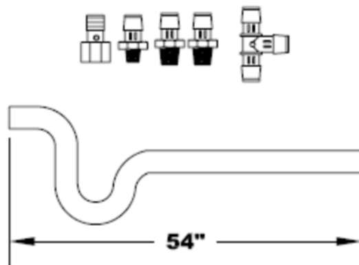
Universal Condensate Hose Kit with P-Trap, End Fittings, Blow Down Valve Fitting and Tee
